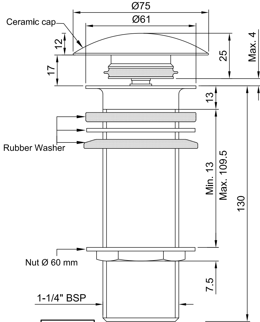
SIDE VIEW
