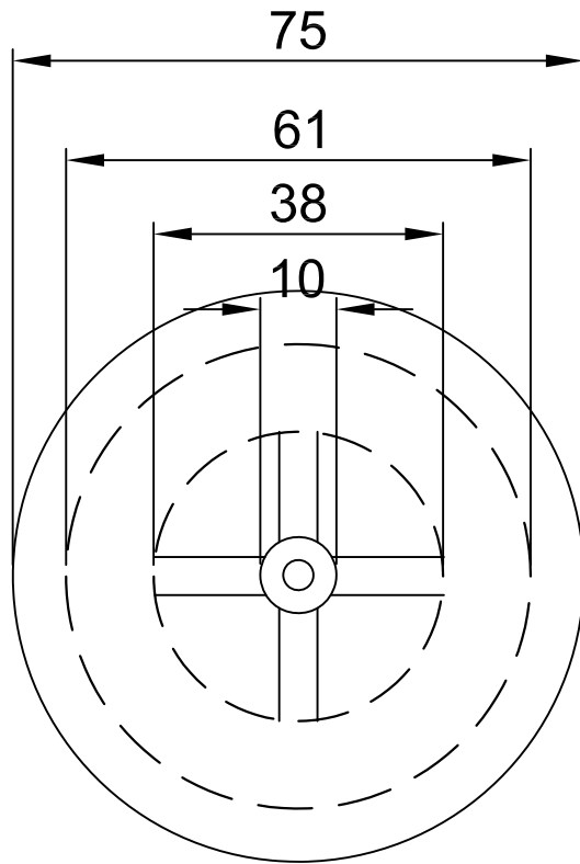
TOP VIEW
